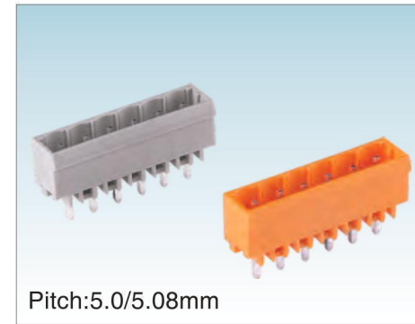
Pitch:5.0/5.08mm
