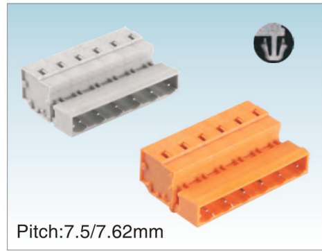
Pitch:7.5/7.62mm
