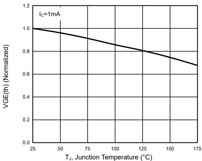
Figure 11 Gate-Emitter Threshold Voltage as a Function of Junction Temperature(Normalized)
